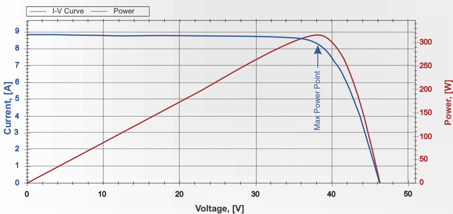
I-V MEASUREMENT
